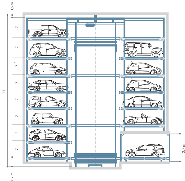
Free standing steel structure, above ground
